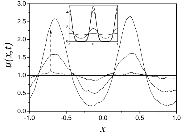
FIGURE 1. Typical stochastic evolution of the field u(x, t) . The initial condition is u(x, 0) \equiv u_0 = 1 and the evolution follows Eq.(2.1) with \epsilon = 10^{-2} . The physical parameters (a, b, D, w, L) are chosen in such a way the initial condition is unstable (see Tables I and II). The arrow shows the amplitude of the stochastic evolution at three different times: t = (10, 20, 25) , i.e., evolving from the uniform toward the patterned state. The inset shows the time-evolution to the final state from a pure deterministic solution with initial condition: u(x, 0) = 1 + \sqrt{\epsilon} \cos(k_e x) for the set of times: t = (10, 20, 30) .
